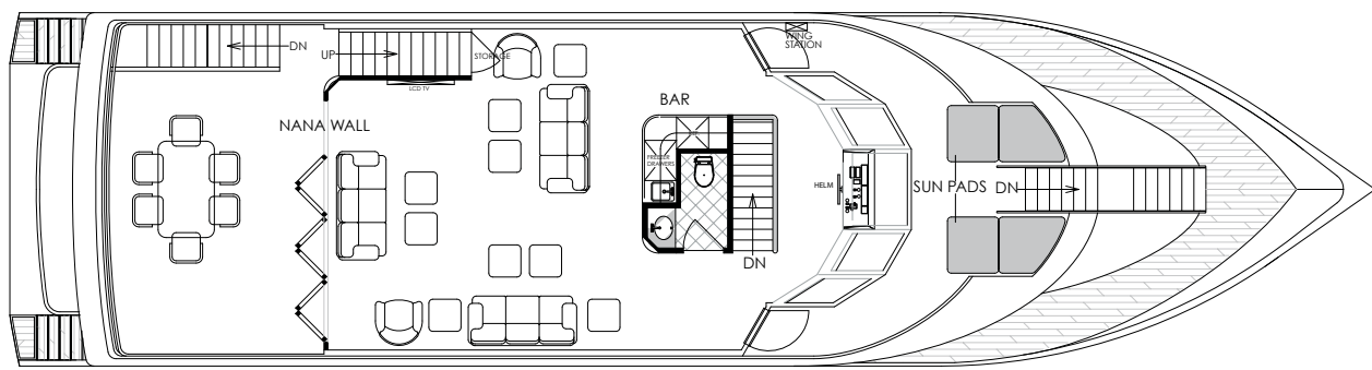
UPPER DECK ARRANGEMENT
